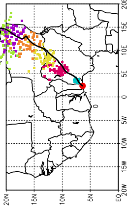
Ballons laches a J+90 h (14/07, 18 UTC)
