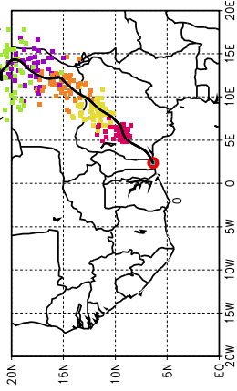
Ballons laches a J+96 h (15/07, 00 UTC)
