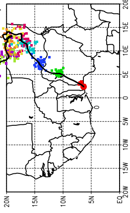
Ballons laches a J+18 h (12/07, 6 UTC)
