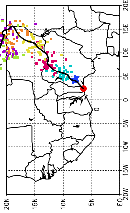
Ballons laches a J+60 h (14/07, 00 UTC)
