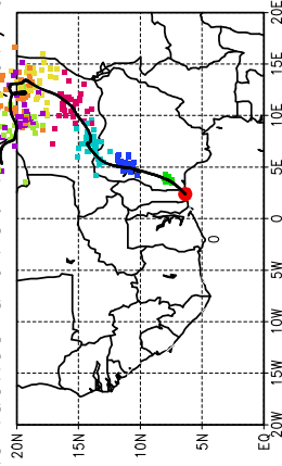
Ballons laches a J+36 h (13/07, 00 UTC)
