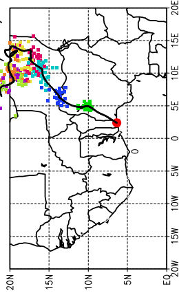
Ballons laches a J+24 h (12/07, 12 UTC)
