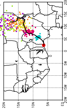
Ballons laches a J+78 h (16/07, 6 UTC)
