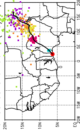
Ballons laches a J+90 h (18/07, 6 UTC)
