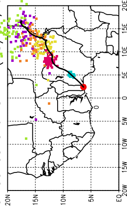
Ballons laches a J+84 h (18/07, 00 UTC)
