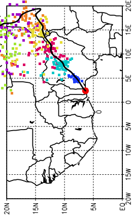
Ballons laches a J+60 h (19/07, 00 UTC)
