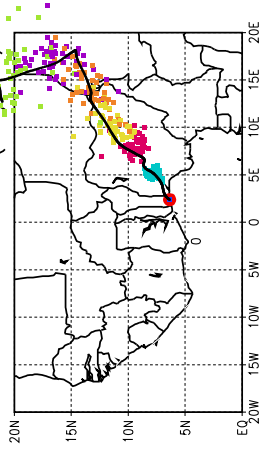
Ballons laches a J+72 h (27/07, 00 UTC)
