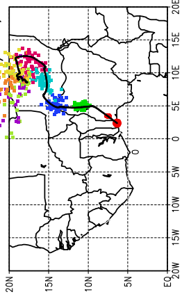
Ballons laches a J+18 h (24/07, 18 UTC)
