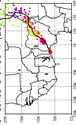
Ballons laches a J+96 h (28/07, 00 UTC)
