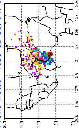
Previs Meteo Proba du 30/04, 00 UTC
