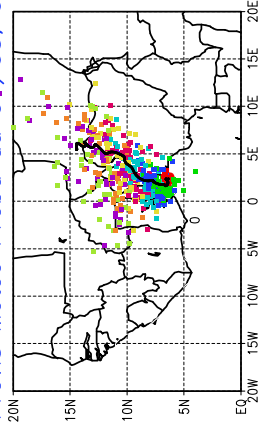
Ballons laches le 01/05/2006 (12 UTC), P = 850hPa Previs Meteo Proba du 01/05, 00 UTC
