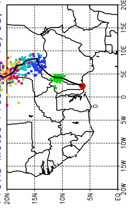
Ballons laches le 16/05/2000 (12 UTC), P = 925hPa Previs Meteo Prob. 15/05, 12 UTC
