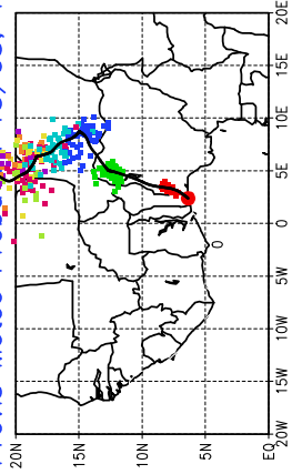
Ballons laches le 16/05/2000 (00 UTC), P = 925hPa Previs Meteo Prob. 15/05, 12 UTC
