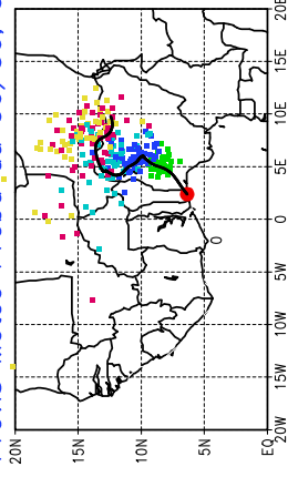
Previs Meteo Proba du 06/06, 00 UTC
