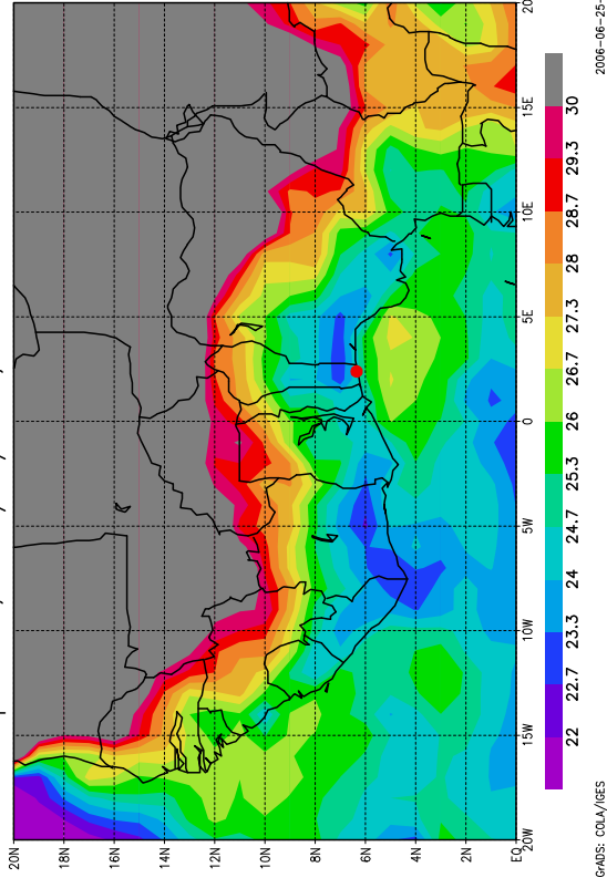
Temperature, le 25/06/2006, Pression = 1000hPa
