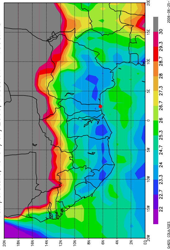
Temperature, le 01/07/2006, Pression = 1000hPa
