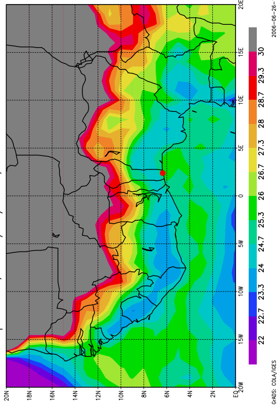
Temperature, le 28/06/2006, Pression = 1000hPa
