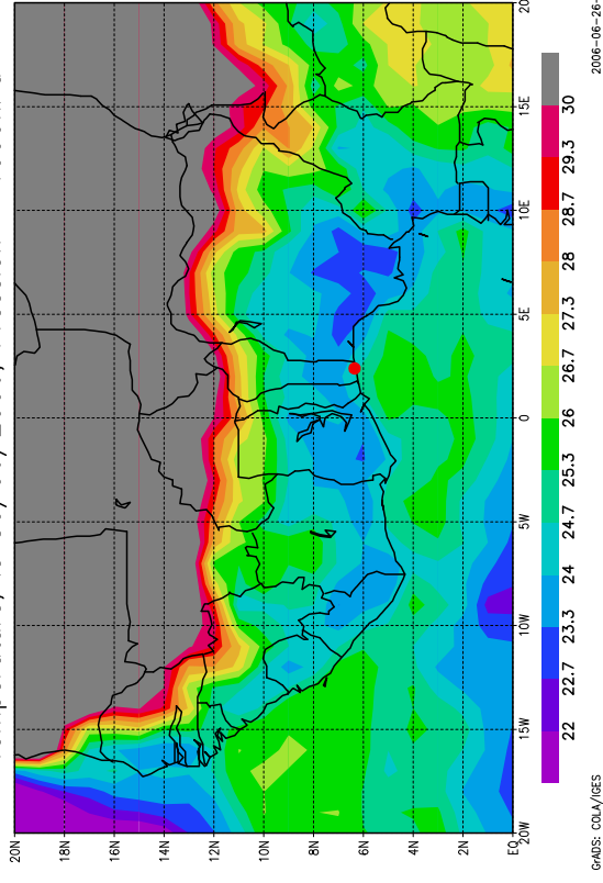
Temperature, le 30/06/2006, Pression = 1000hPa
