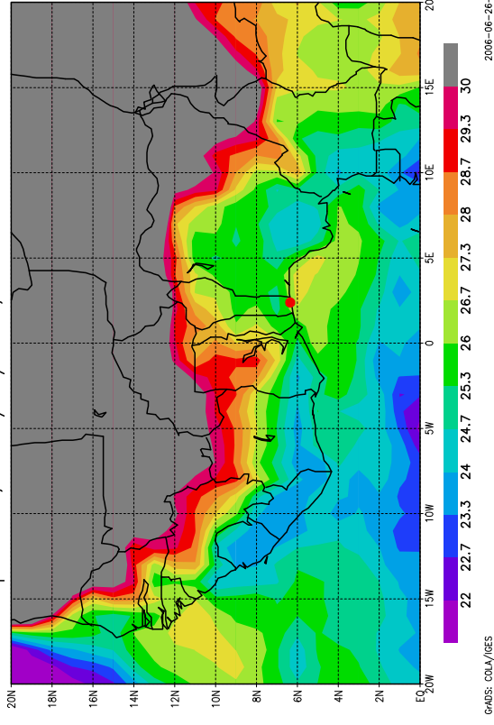
Temperature, le 26/06/2006, Pression = 1000hPa
