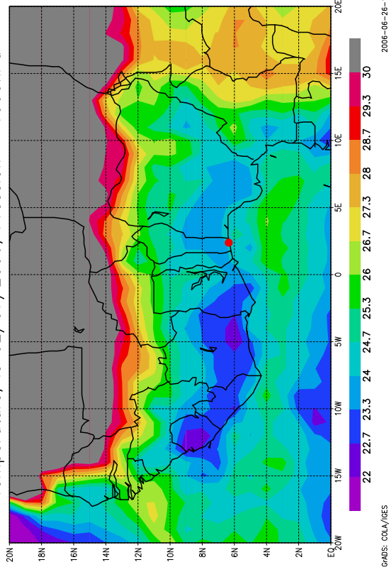
Temperature, le 02/07/2006, Pression = 1000hPa
