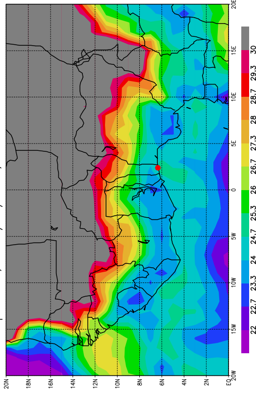
Temperature, le 11/07/2006, Pression = 1000hPa
