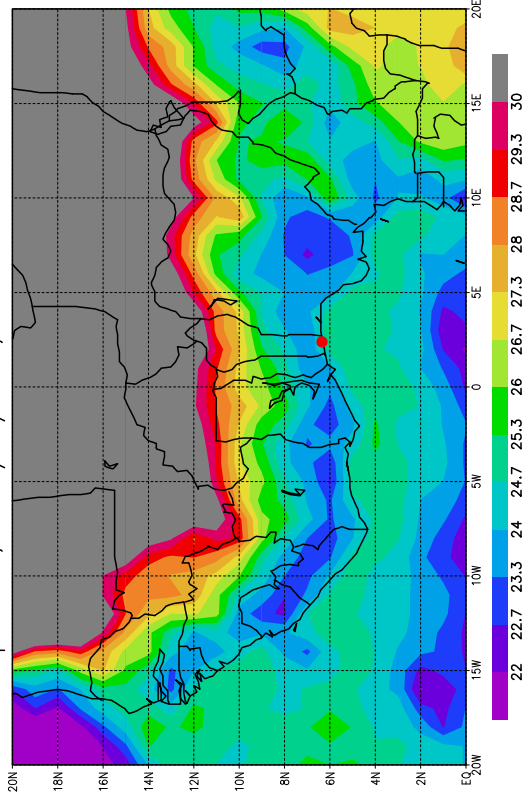
Temperature, le 13/07/2006, Pression = 1000hPa
