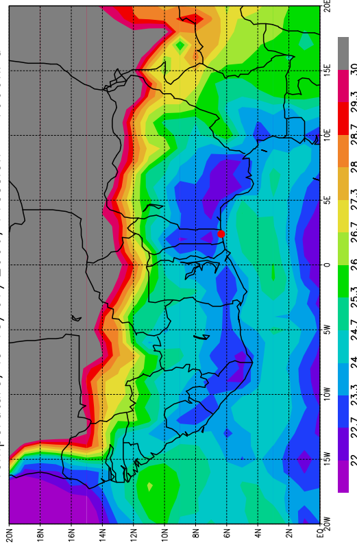
Temperature, le 15/07/2006, Pression = 1000hPa
