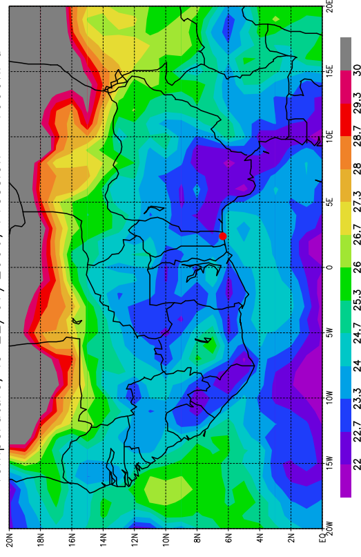
Temperature, le 22/07/2006, Pression = 1000hPa
