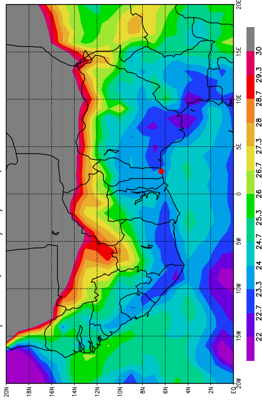
Temperature, le 18/07/2006, Pression = 1000hPa
