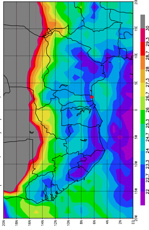
Temperature, le 21/07/2006, Pression = 1000hPa
