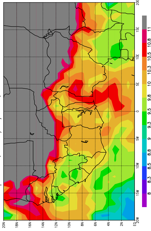
Temperature, le 28/06/2006, Pression = 700hPa
