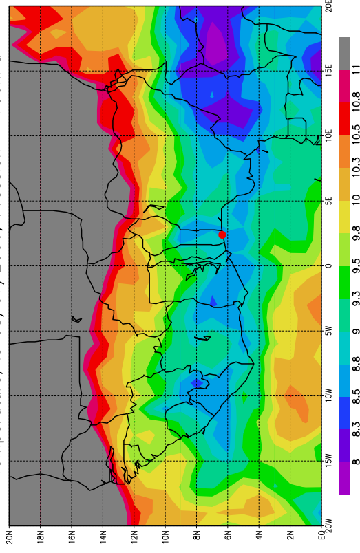
Temperature, le 08/07/2006, Pression = 700hPa
