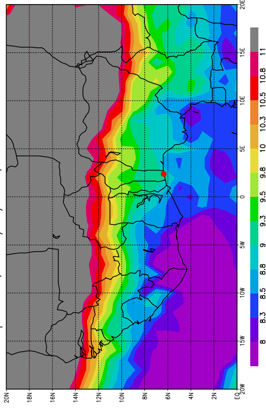
Temperature, le 06/07/2006, Pression = 700hPa
