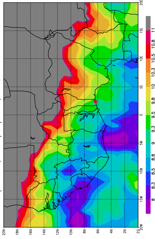
Temperature, le 04/07/2006, Pression = 700hPa
