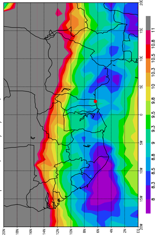
Temperature, le 07/07/2006, Pression = 700hPa
