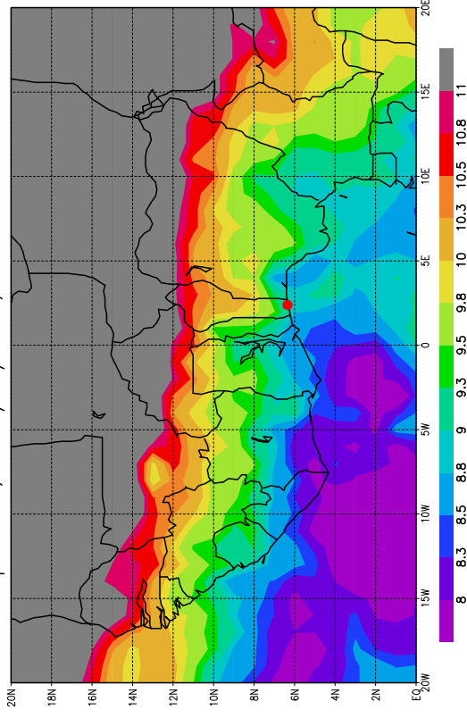
Temperature, le 05/07/2006, Pression = 700hPa
