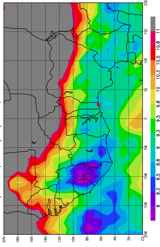
Temperature, le 16/07/2006, Pression = 700hPa
