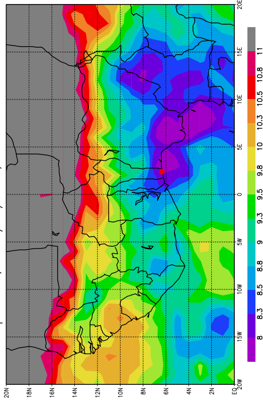
Temperature, le 25/07/2006, Pression = 700hPa
