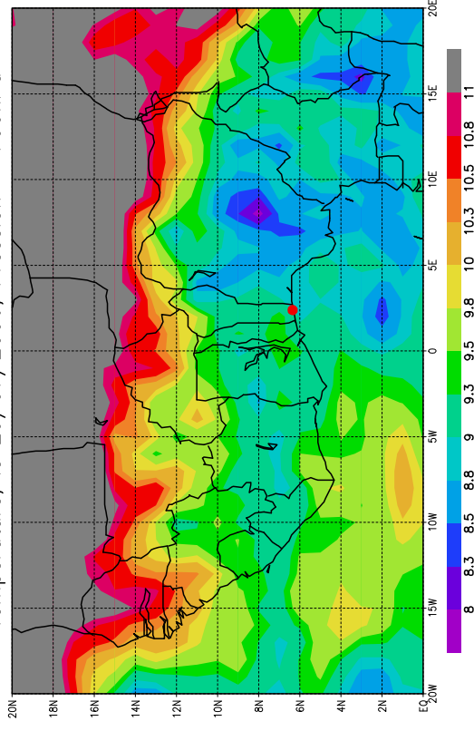
Temperature, le 29/07/2006, Pression = 700hPa
