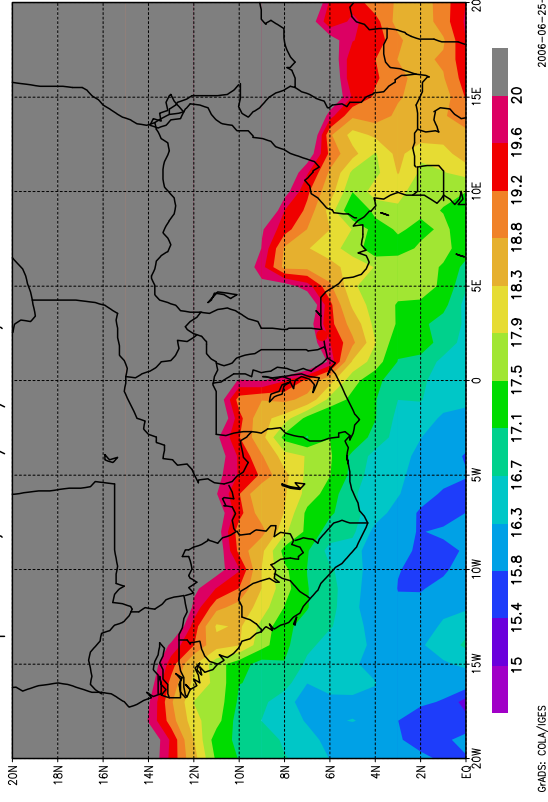
Temperature, le 25/06/2006, Pression = 850hPa
