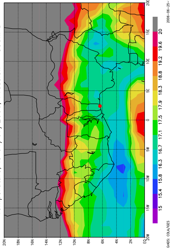
Temperature, le 01/07/2006, Pression = 850hPa
