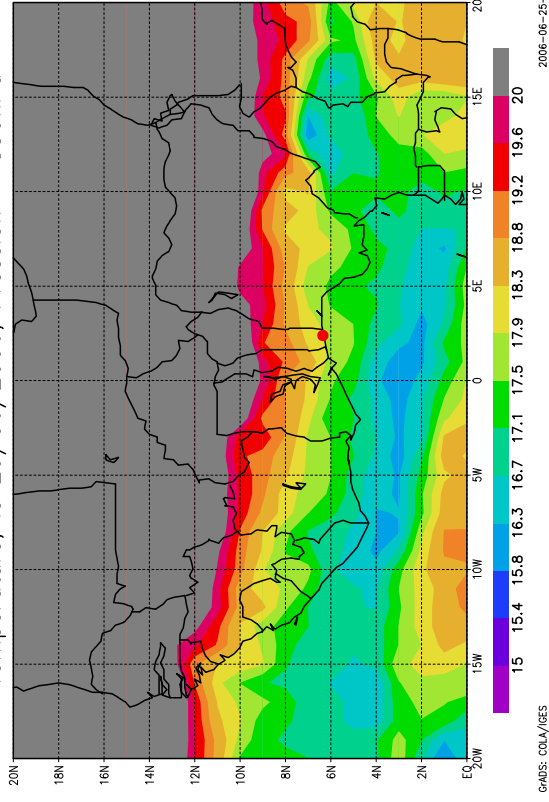
Temperature, le 29/06/2006, Pression = 850hPa
