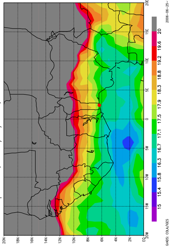
Temperature, le 27/06/2006, Pression = 850hPa
