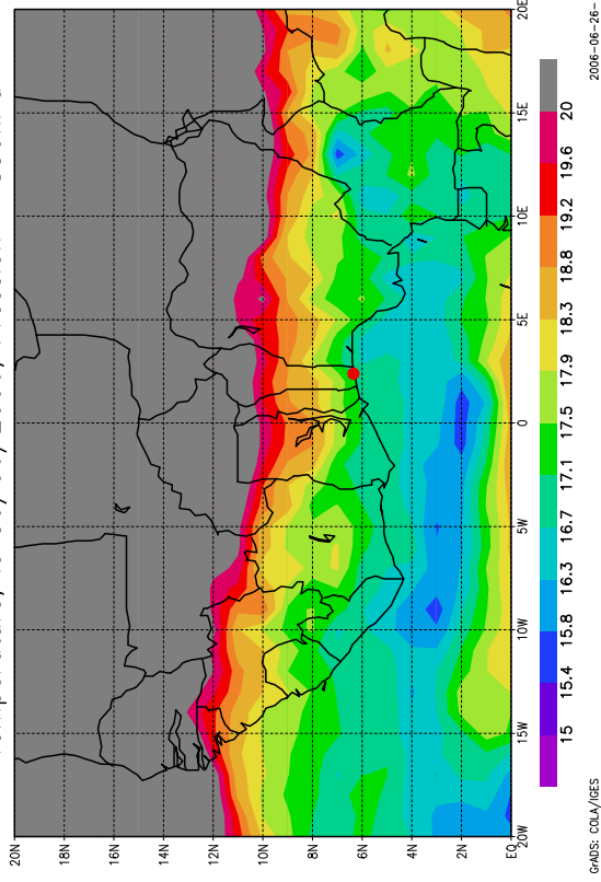
Temperature, le 30/06/2006, Pression = 850hPa
