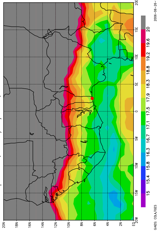
Temperature, le 28/06/2006, Pression = 850hPa
