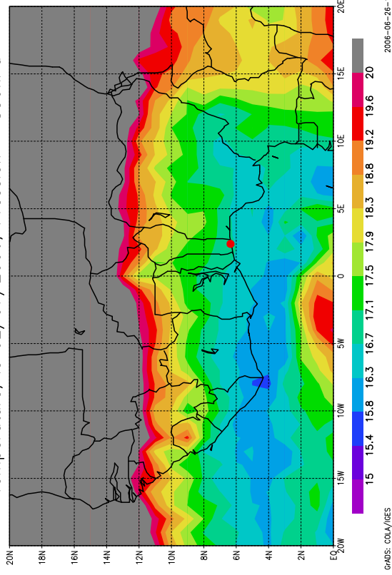
Temperature, le 02/07/2006, Pression = 850hPa
