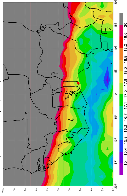
Temperature, le 29/06/2006, Pression = 850hPa
