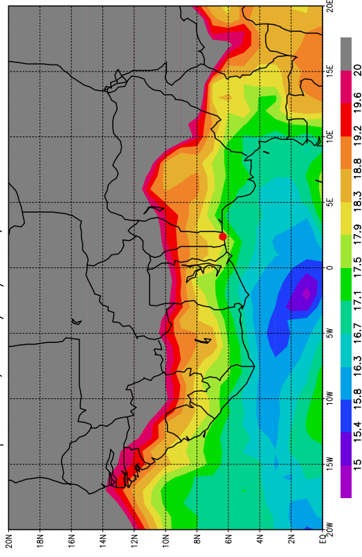
Temperature, le 27/06/2006, Pression = 850hPa
