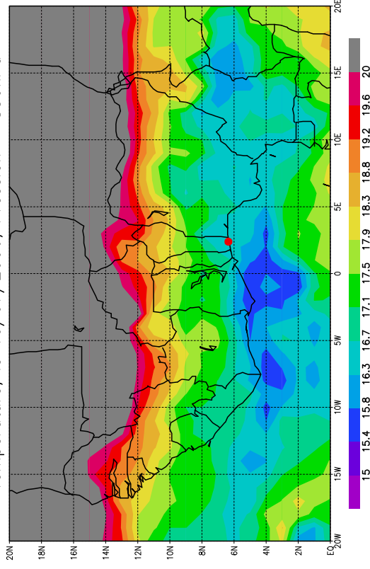
Temperature, le 10/07/2006, Pression = 850hPa
