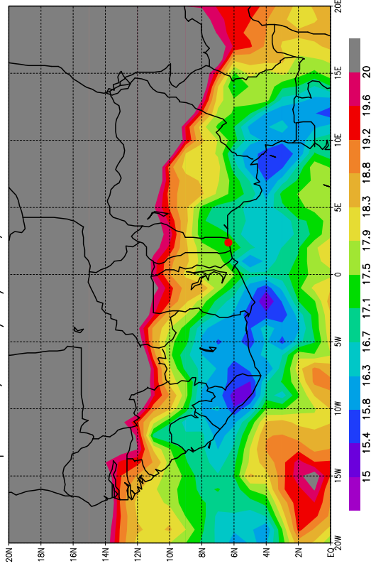
Temperature, le 06/07/2006, Pression = 850hPa
