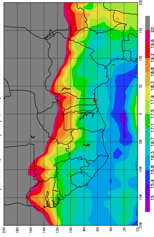
Temperature, le 16/07/2006, Pression = 850hPa
