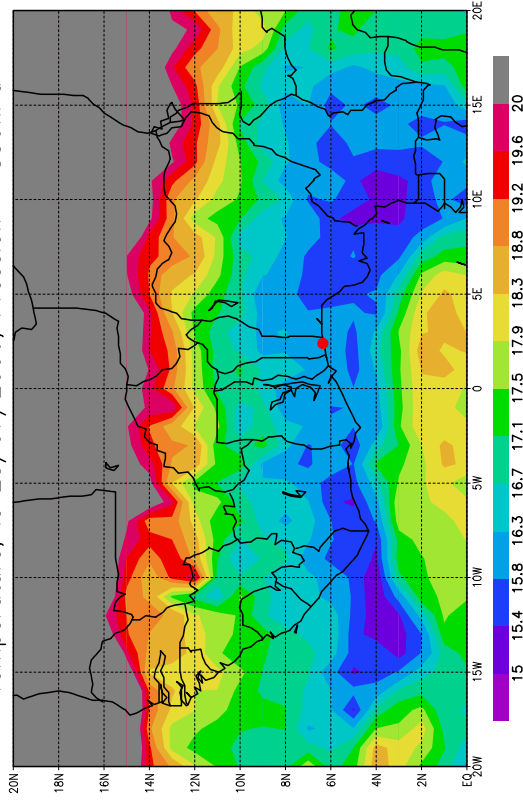
Temperature, le 23/07/2006, Pression = 850hPa
