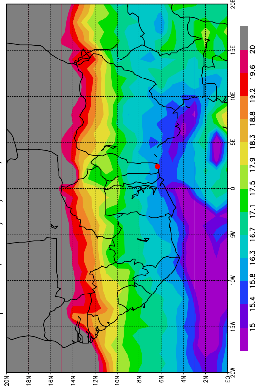
Temperature, le 24/07/2006, Pression = 850hPa
