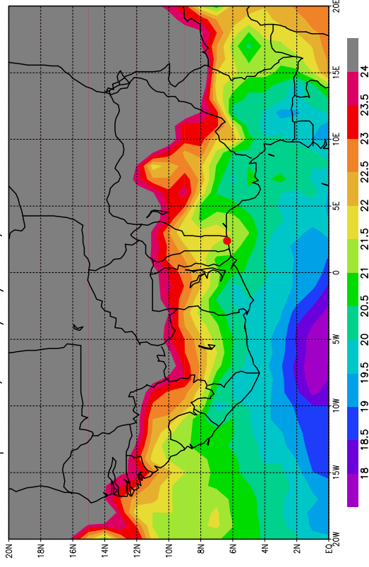
Temperature, le 27/06/2006, Pression = 925hPa
