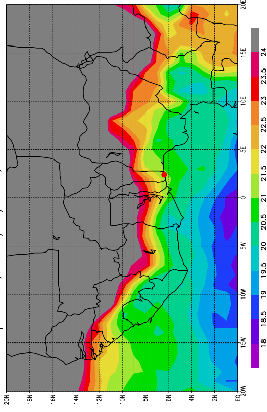
Temperature, le 29/06/2006, Pression = 925hPa
