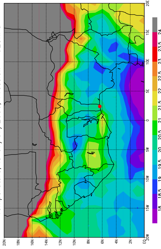
Temperature, le 07/07/2006, Pression = 925hPa
