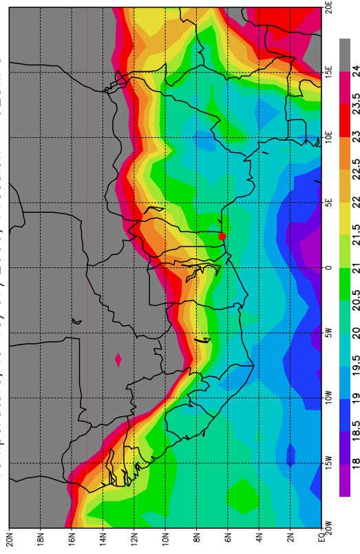
Temperature, le 13/07/2006, Pression = 925hPa
