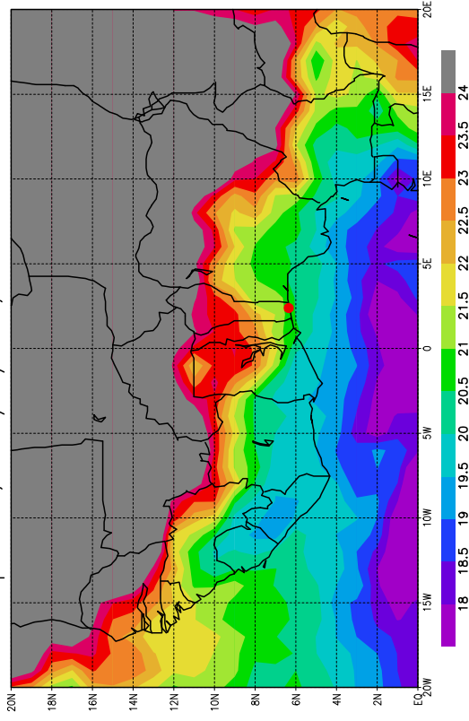
Temperature, le 09/07/2006, Pression = 925hPa
