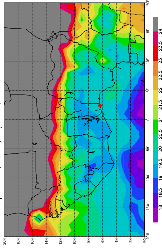
Temperature, le 15/07/2006, Pression = 925hPa
