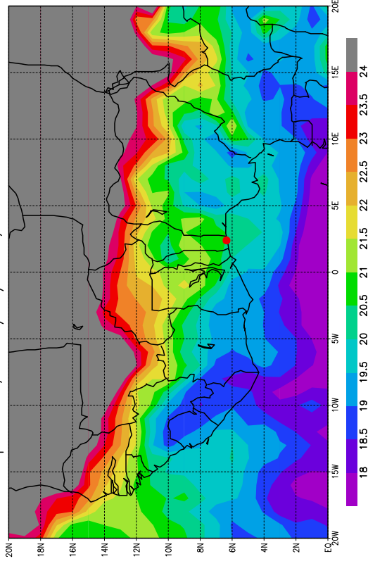
Temperature, le 21/07/2006, Pression = 925hPa
