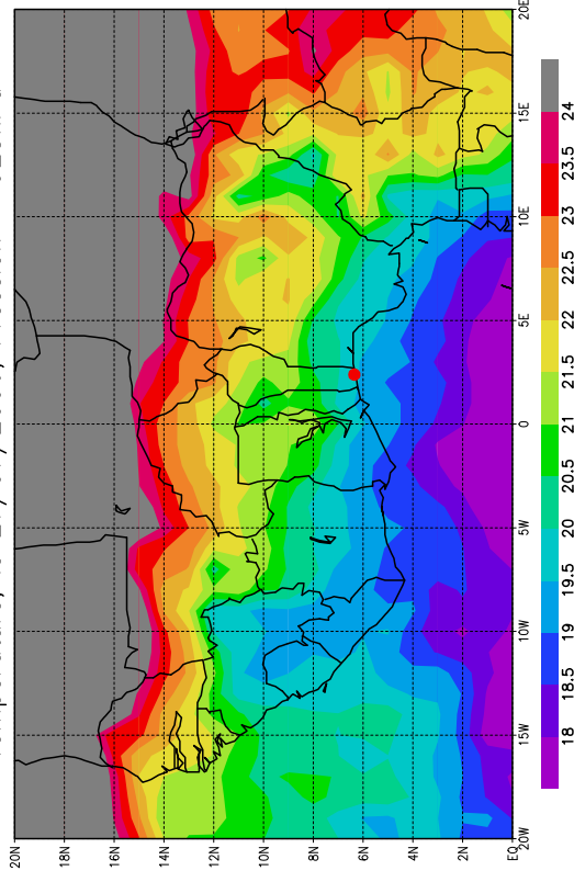
Temperature, le 27/07/2006, Pression = 925hPa
