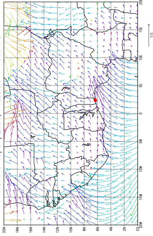
Vent le 16/07/2006, Pression = 1000hPa
