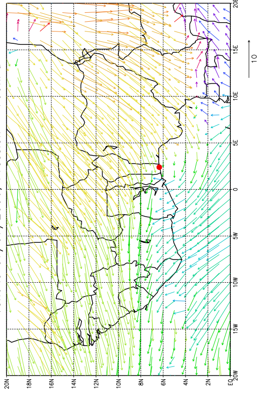
Vent le 07/07/2006, Pression = 700hPa
