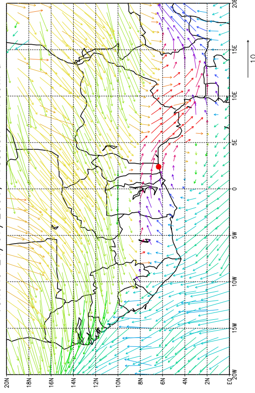
Vent le 21/07/2006, Pression = 700hPa
