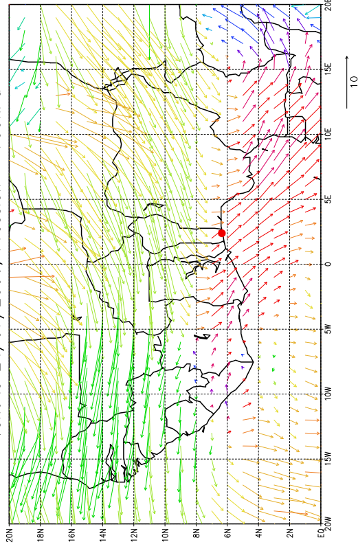
Vent le 24/07/2006, Pression = 700hPa
