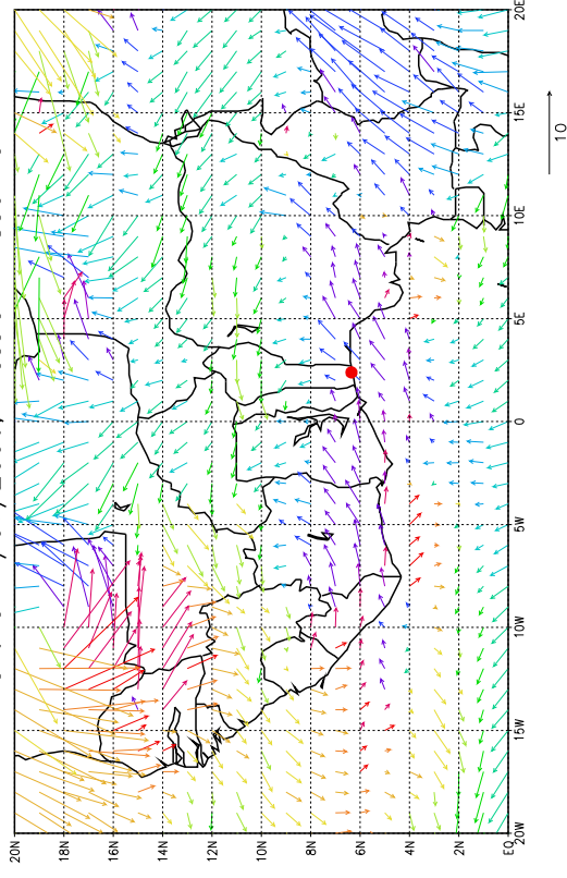
Vent le 11/07/2006, Pression = 850hPa
