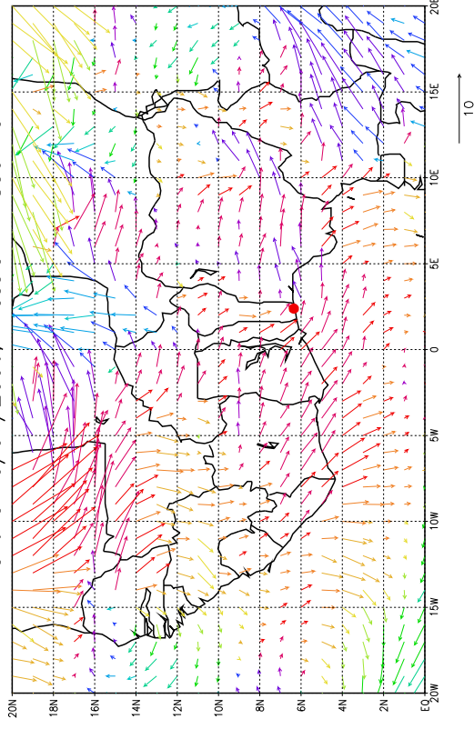
Vent le 10/07/2006, Pression = 850hPa
