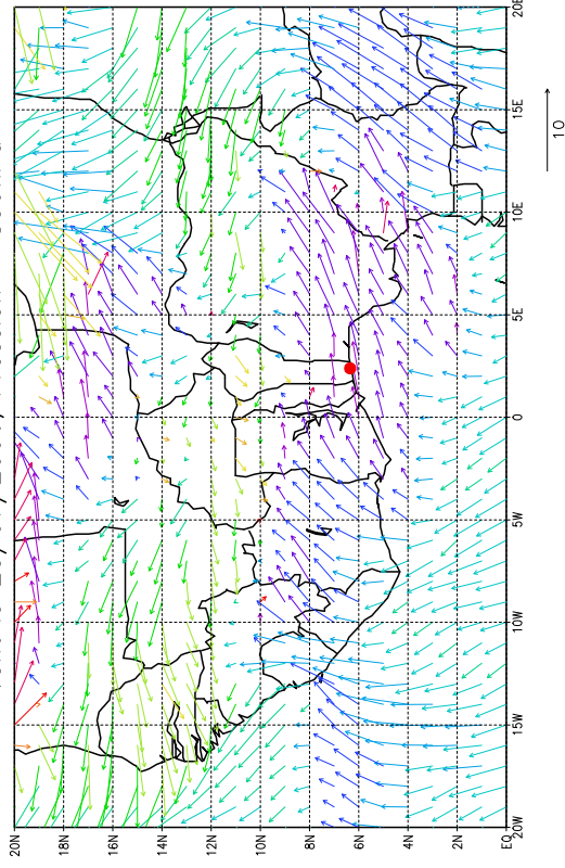
Vent le 25/07/2006, Pression = 850hPa
