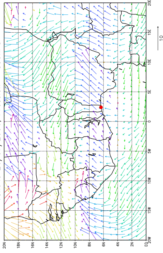
Vent le 26/07/2006, Pression = 850hPa
