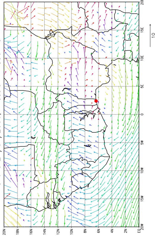
Vent le 27/07/2006, Pression = 850hPa
