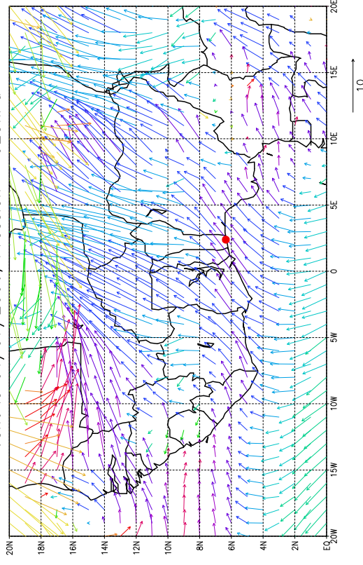
Vent le 01/07/2006, Pression = 925hPa
