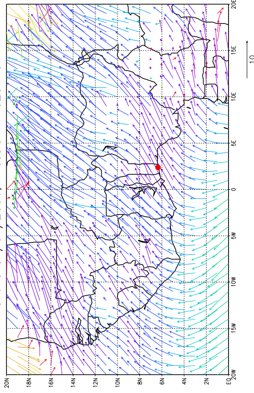
Vent le 04/07/2006, Pression = 925hPa
