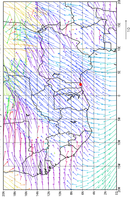
Vent le 09/07/2006, Pression = 925hPa
