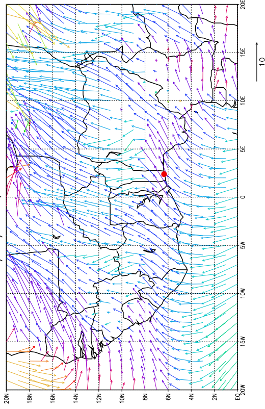
Vent le 15/07/2006, Pression = 925hPa
