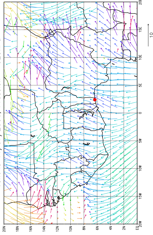
Vent le 11/07/2006, Pression = 925hPa
