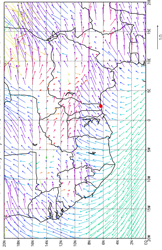
Vent le 28/07/2006, Pression = 925hPa
