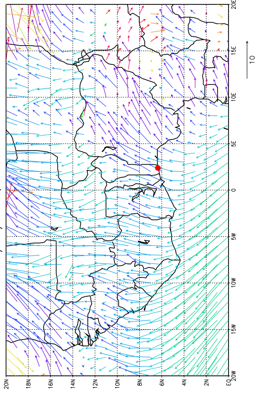
Vent le 27/07/2006, Pression = 925hPa
