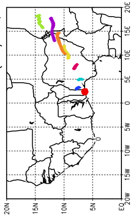
Ballons laches a J+60 h (26/07, 12 UTC)
