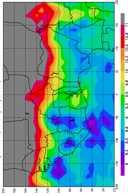
Temperature, le 30/07/2006, Pression = 700hPa
