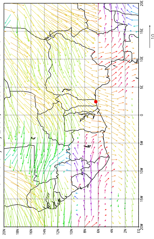
Vent le 31/07/2006, Pression = 700hPa
