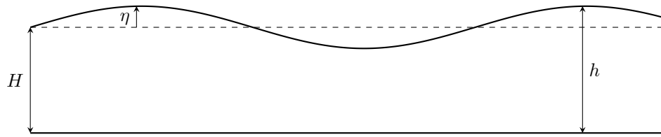
Figure 2.2: The Shallow water model. H is the mean depth of the fluid, h is its actual depth and \eta the surface height anomaly: h = H + \eta .
