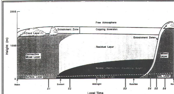
Fig. 1.7 The boundary layer in high pressure regions over land consists of three major parts: turbulent mixed layer; a less-turbulent residual layer containing former mixed-layer air; and a nocturnal stable boundary layer of sporadic turbulence. The mixed layer can be subdivided into a cloud layer and a subcloud layer. Time markers indicated by S1-S6 will be used in Fig. 1.12.
