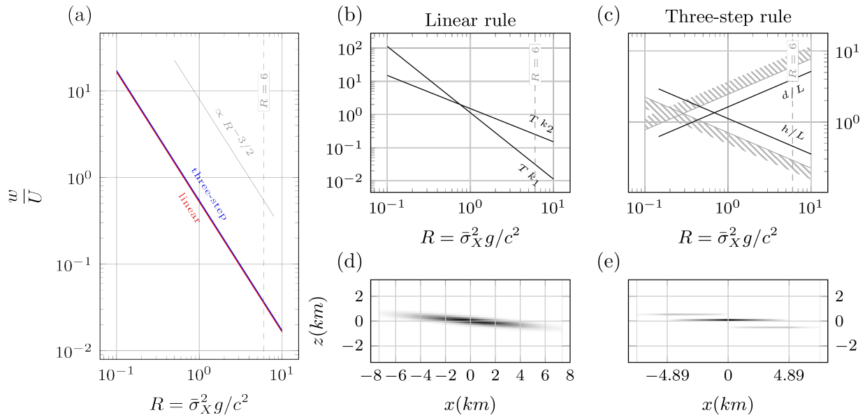
Fig. 4. Comparison of control rules: (a) control cost w = \mathbf{E}[|u_1|] as a function of the dimensionless parameter R for the two different control rules; the two control costs are almost indistinguishable, differing by less than 5%. (b,c) Control parameters and (d,e) corresponding probability density for the hurricane case ( R = 6 ) for the linear and TLC control rules. Gray patterns in (c) define the limit of each curve for which a given value of R is attainable, given by (14).
