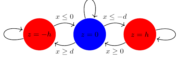
Fig. 2. Implementation of the three-level control rule.
