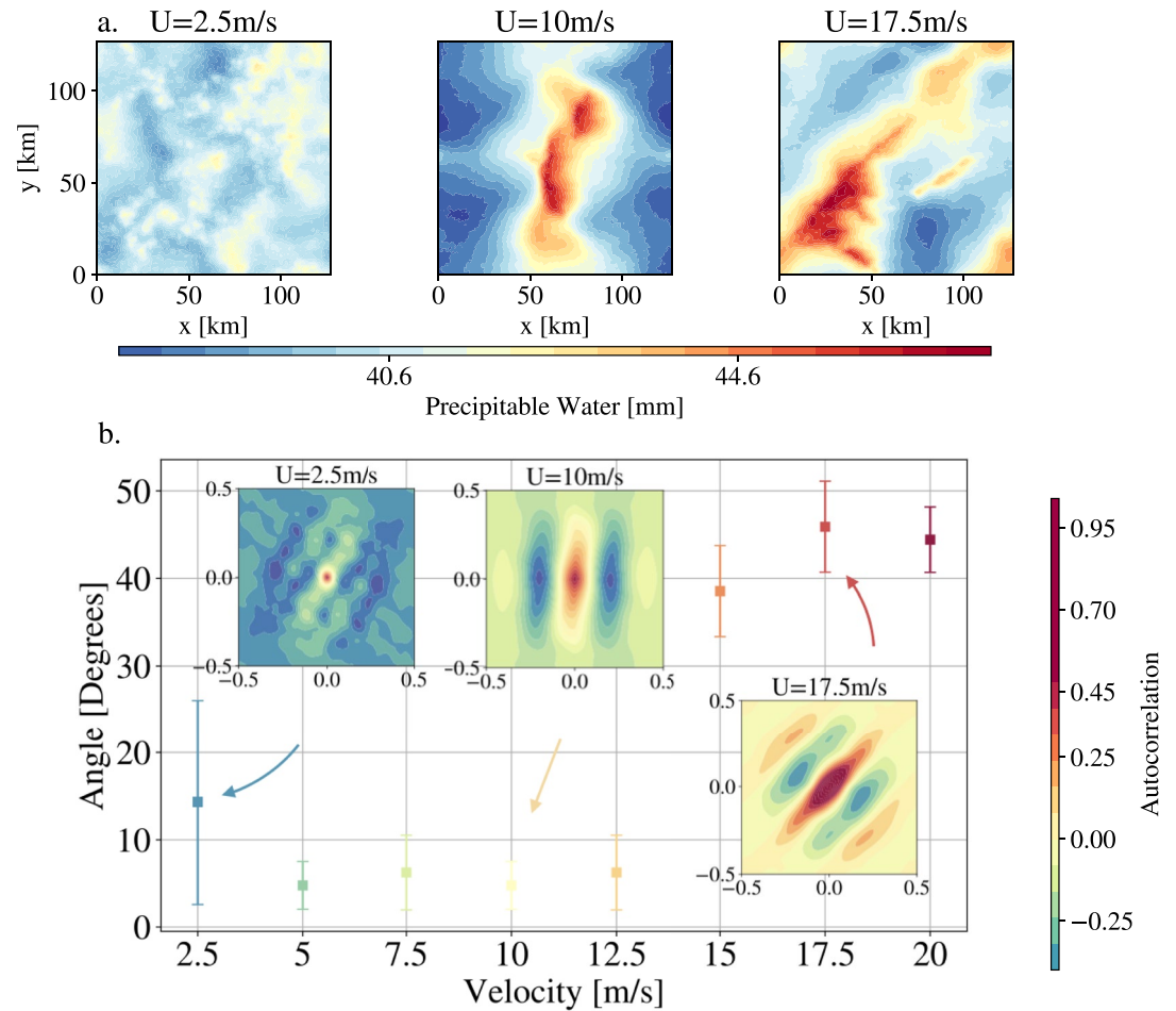
Figure 2. (a) Snapshots (31st day) of the spatial distribution of Precipitable Water (PW) for different shear values. In the absence of shear, no squall lines are observed. For U_{\text{sc}} = 10 \text{ m s}^{-1} , arcs perpendicular to the wind, that is, parallel to the y -axis, are formed. For U_{\text{sc}} = 17.5 \text{ m s}^{-1} , the squall line is oriented with respect to the y -axis. (b) Results of the automatic method based on PW autocorrelation developed in this paper to detect the angle a between the squall line and the y -axis. The auto-correlations of PW corresponding to the three top snapshots are also displayed; they are normalized and the colorbar is saturated to highlight the correlation areas.
