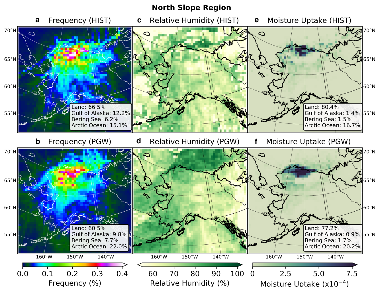
Fig. 3 Results of the backward tracking analysis for the parcels released in the North Slope's convective storms. a Normalized parcel track density on a coarse grid of the model domain. c Mean relative
