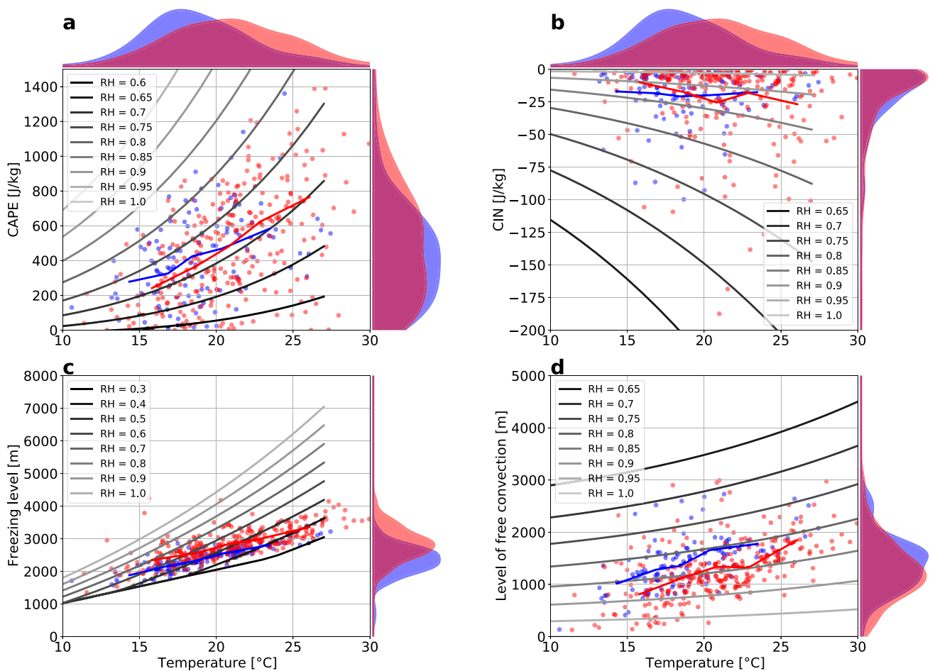
Fig. 7 Scatter plot of temperature and a CAPE, b CIN, c freezing level height, d LFC height. Each point represents the environment of one storm in the control (blue points) and PGW (red points) simulation. Solid blue and red lines respectively correspond to the centroids of blue and red points binned by temperature with bin edges defined as the 10th, 30th, 50th, 70th and 90th percentiles of the temperature distribution. Solid gray lines show the relationship expected from the
