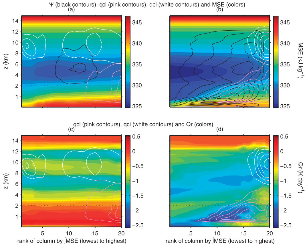
FIG. 11. (a),(b) Daily mean circulation and (c),(d) radiative cooling after 8 days (a),(c) in a run with disorganized convection and (b),(d) in a run that self-aggregates. Note the stretched vertical coordinate z below 2 km. In (a) and (b), black contours show the streamfunction \Psi (contour interval = 20 \text{ kg s}^{-1} starting at \pm 20 \text{ kg s}^{-1} ; solid for negative values and dashed for positive values) as a function of vertically integrated moist static energy and height z . In all panels, pink and white contours show nonprecipitating condensate amounts for liquid and ice, respectively (contour interval = 5 \text{ mg kg}^{-1} starting at 5 \text{ mg kg}^{-1} ). The background colors represent moist static energy and radiative cooling in the top and bottom rows, respectively. Both runs have a domain size of 254 km, a resolution of 2 km, homogenized surface fluxes, homogenized SW radiative cooling, and homogenized longwave radiative cooling from water vapor. In addition, the simulation shown in (a) and (c) has homogenized radiative cooling from condensates and therefore does not self-aggregate.
