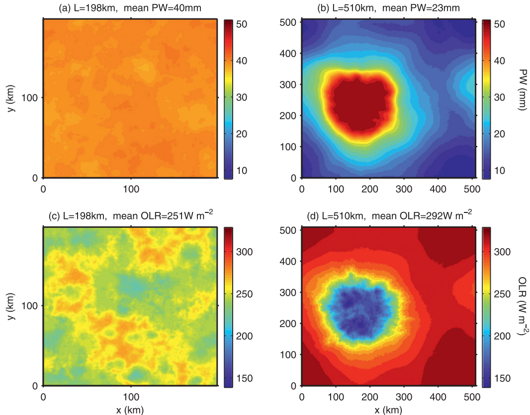
FIG. 2. Daily mean (a),(b) precipitable water (PW) and (c),(d) outgoing longwave radiation (OLR) after 60 days in two simulations with the same resolution dx = 2 \text{ km} but different domain sizes L = (a),(c) 198 and (b),(d) 510 km. Convection self-aggregates when the domain is large enough (Fig. 1b), resulting in a moist region where convection is concentrated, surrounded by air with very dry conditions and strong longwave cooling.
