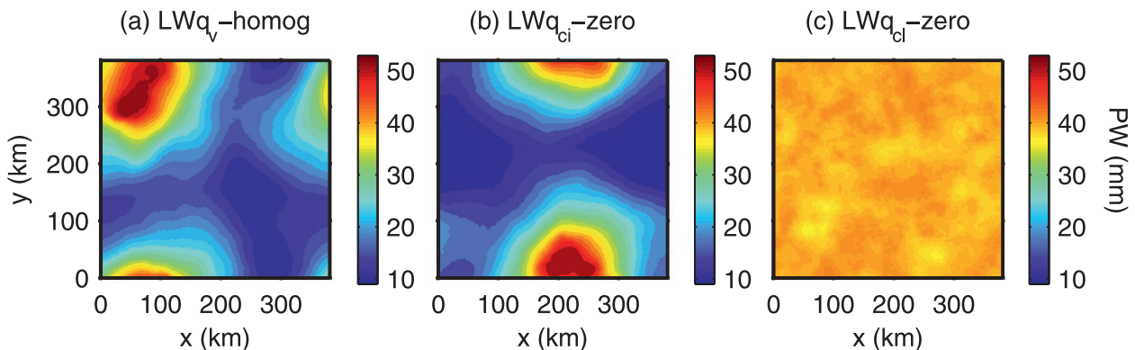
FIG. 10. Daily mean PW (mm) after 30 days in various sensitivity simulations (a) LWq_v -homog, (b) LWq_{ci} -zero, and (c) LWq_{cl} -zero described in Table 1.
